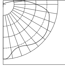
BIS42CCXX-GAB-GEP TEST NUMBER: 26289 LAMP: 42W CFL LUMENS: 3,200 MOUNTING HEIGHT: 12 FEET
