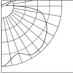
BIS100IXX-GAB-GEP TEST NUMBER: 26245 LAMP: 100W A19 LUMENS: 1,680 MOUNTING HEIGHT: 12 FEET
