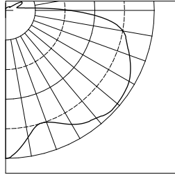
BIS175MXX-GAB-GEP TEST NUMBER: 26238 LAMP: 175W MH, COATED LUMENS: 15,000 MOUNTING HEIGHT: 12 FEET
